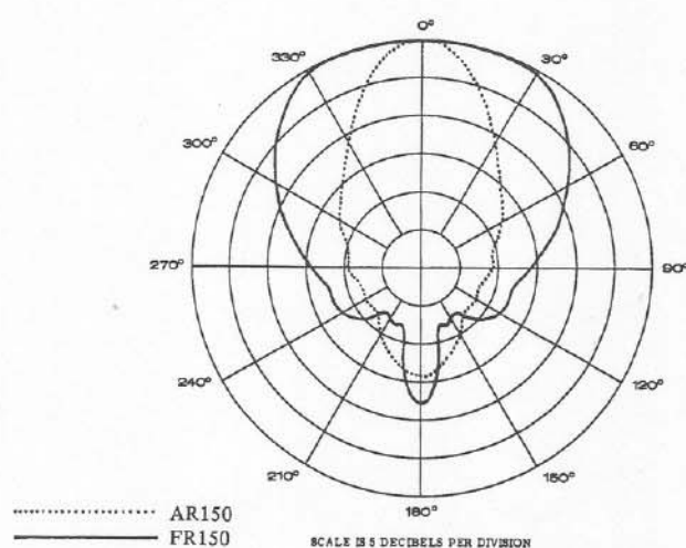
Figure 5 – Polar Response, 700–1300 Hz Sweep Sine Wave (AR150, FR150)
